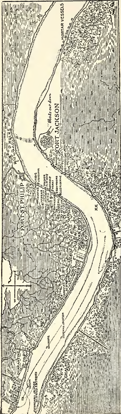
SECTION OF MISSISSIPPI RIVER, SHOWING DEFENCES OF FORTS JACKSON AND ST. PHILIP AT TIME OF BOMBARDMENT.
